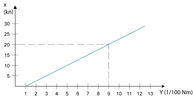
X axis = Boat speed in knots Y axis = Arrival circle, radius in 1/100 Nm
