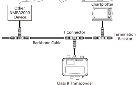
Figure 8 NMEA 2000 Network
