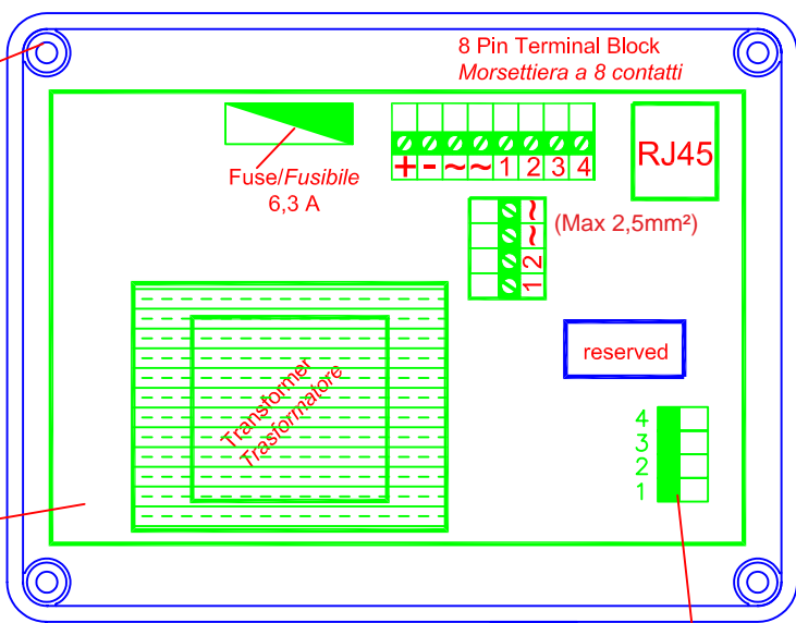
1 HORN HEATING
