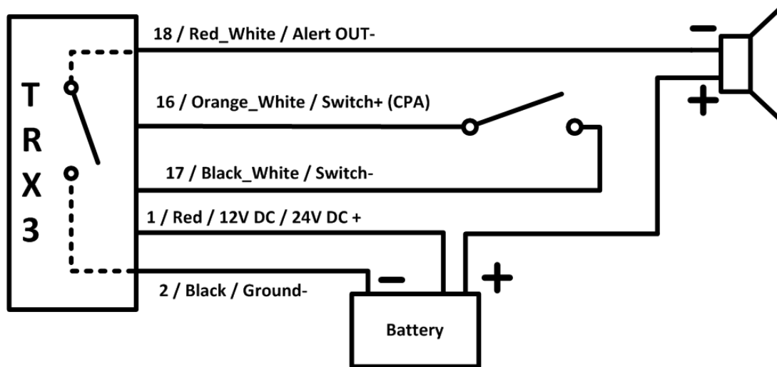
Figure: 4 CPA Alert connection sketch
