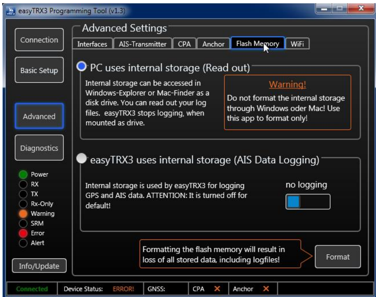
Figure: 28 Memory setting programming tool
