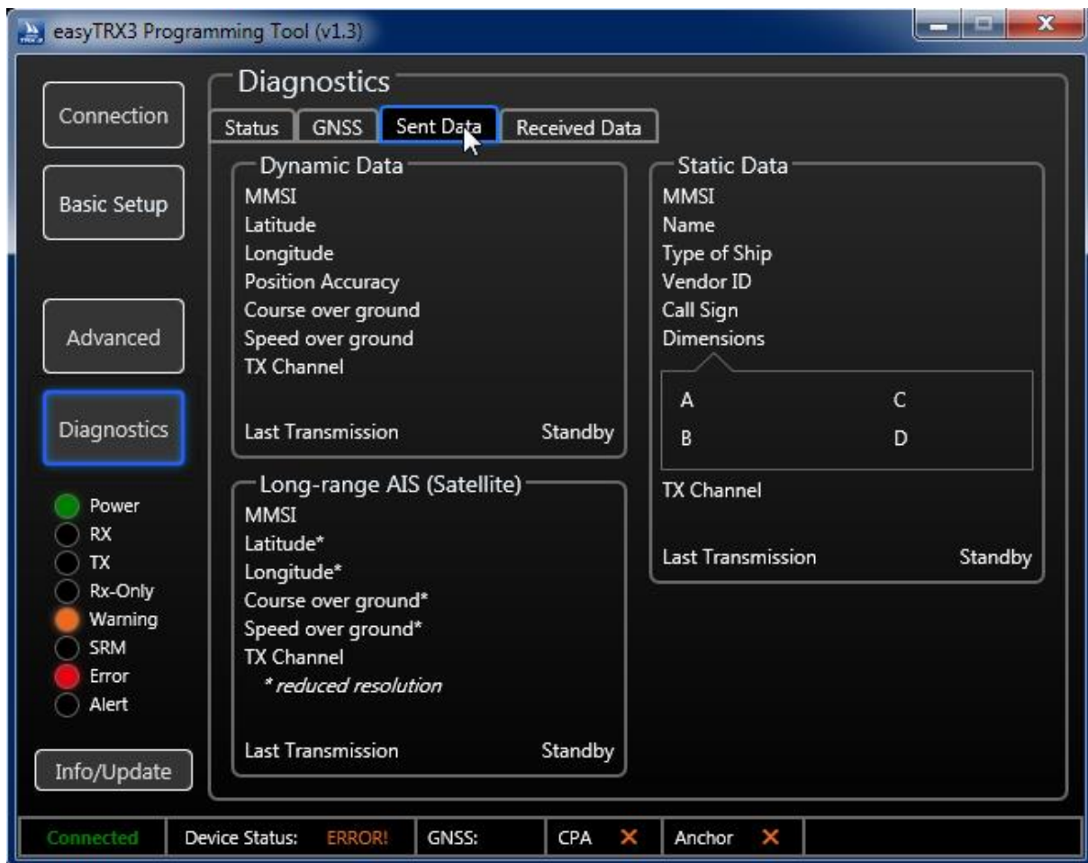
Figure: 47 Sent data screen programming tool
