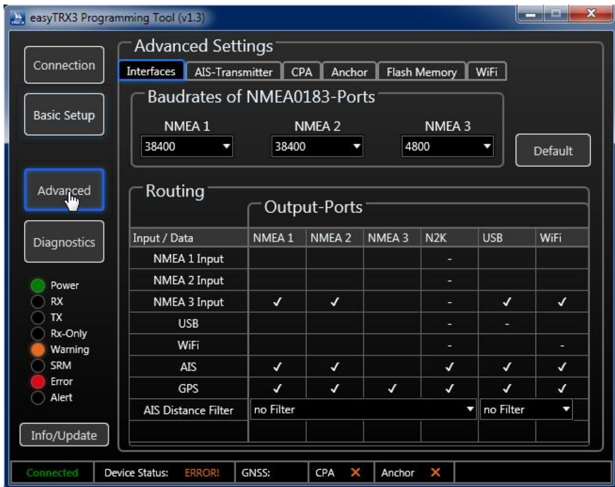
Figure: 16 Advance setting screen programming software
