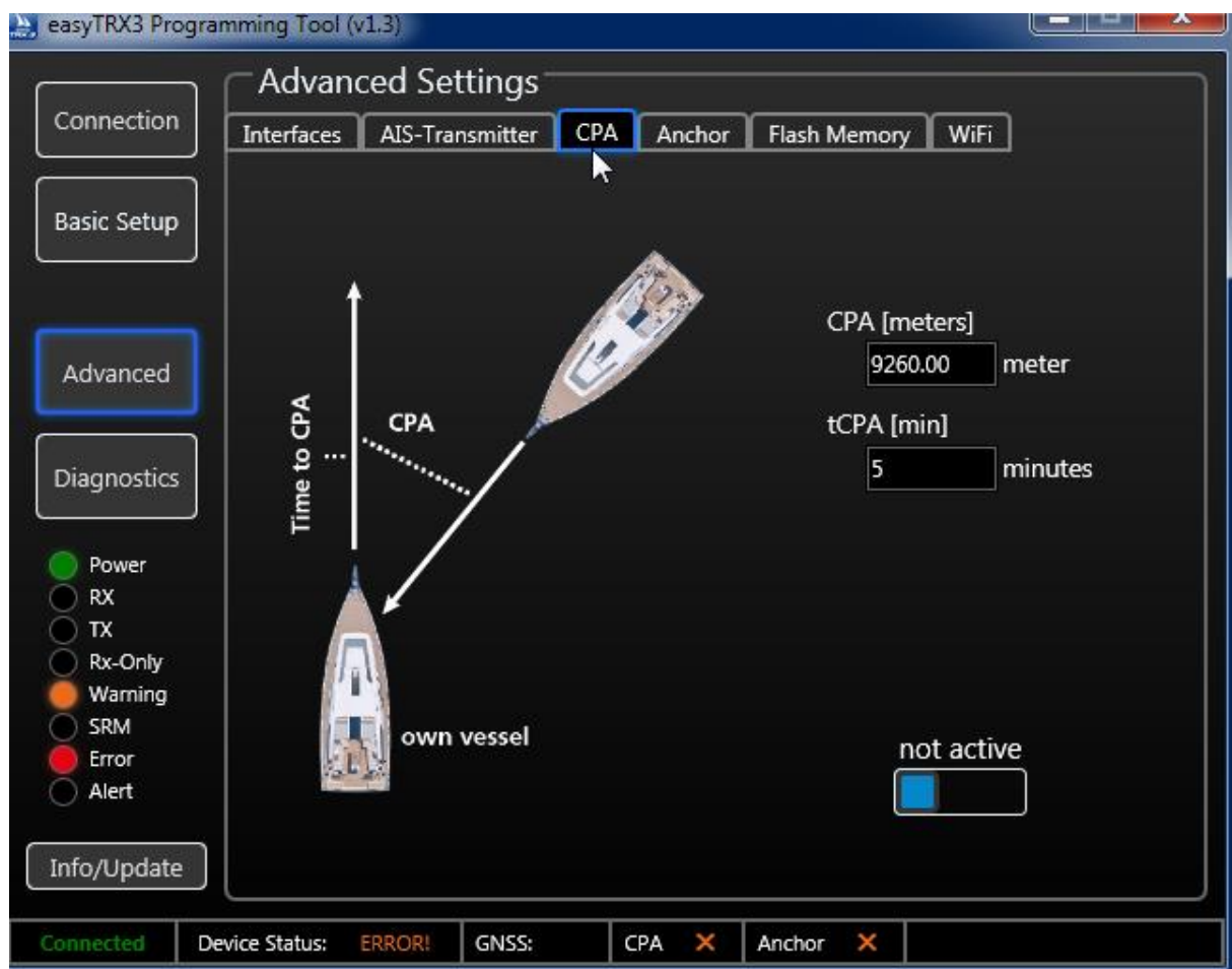
Figure: 24 CPA settings programming tool
