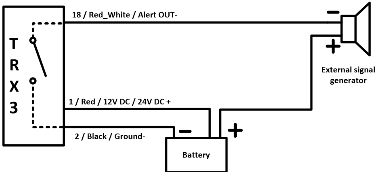
Figure: 7 External signal generator connection sketch
