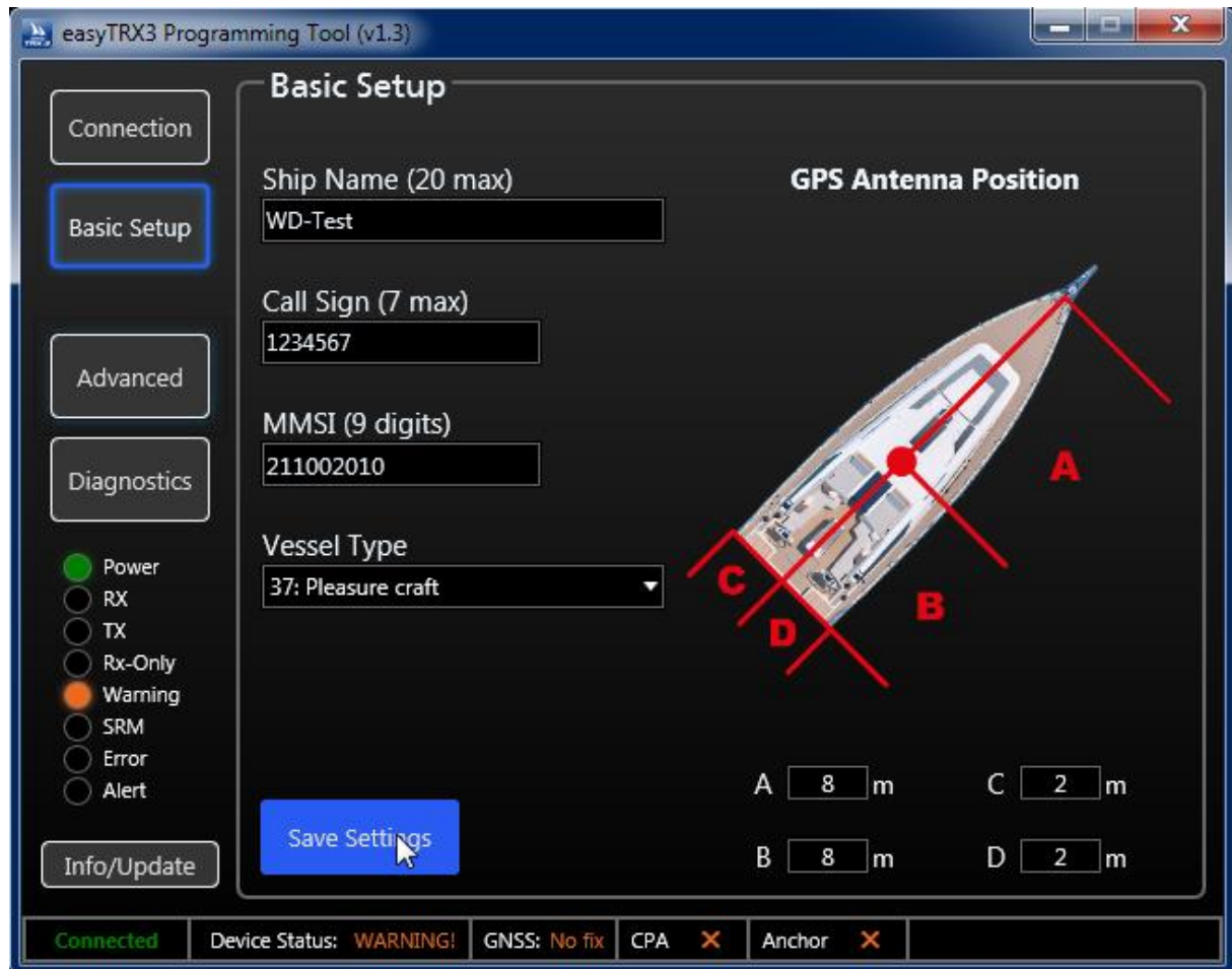
Figure: 14 Basic setup screen programming software
