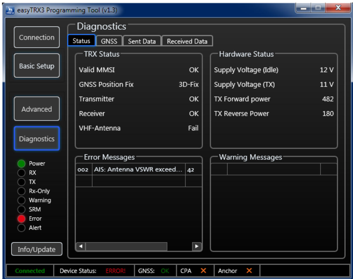
Figure: 45 Diagnostic screen programming tool
