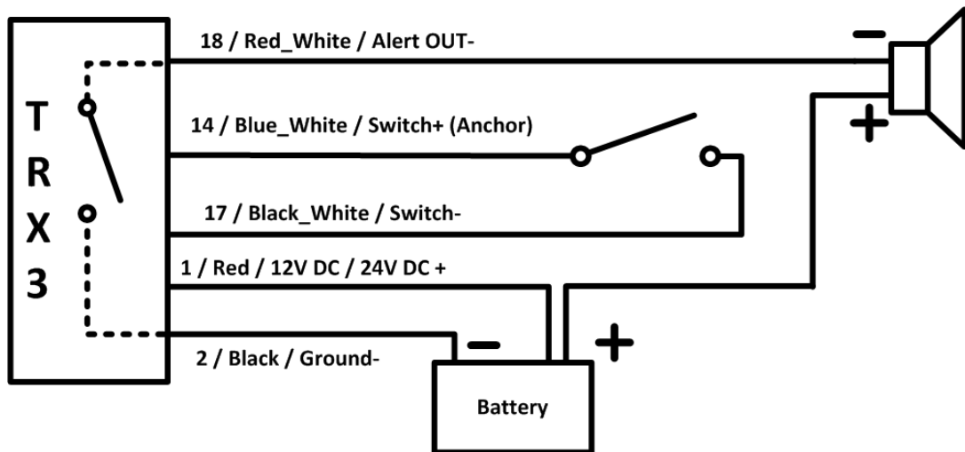
Figure: 5 Anchor Alert connection sketch
