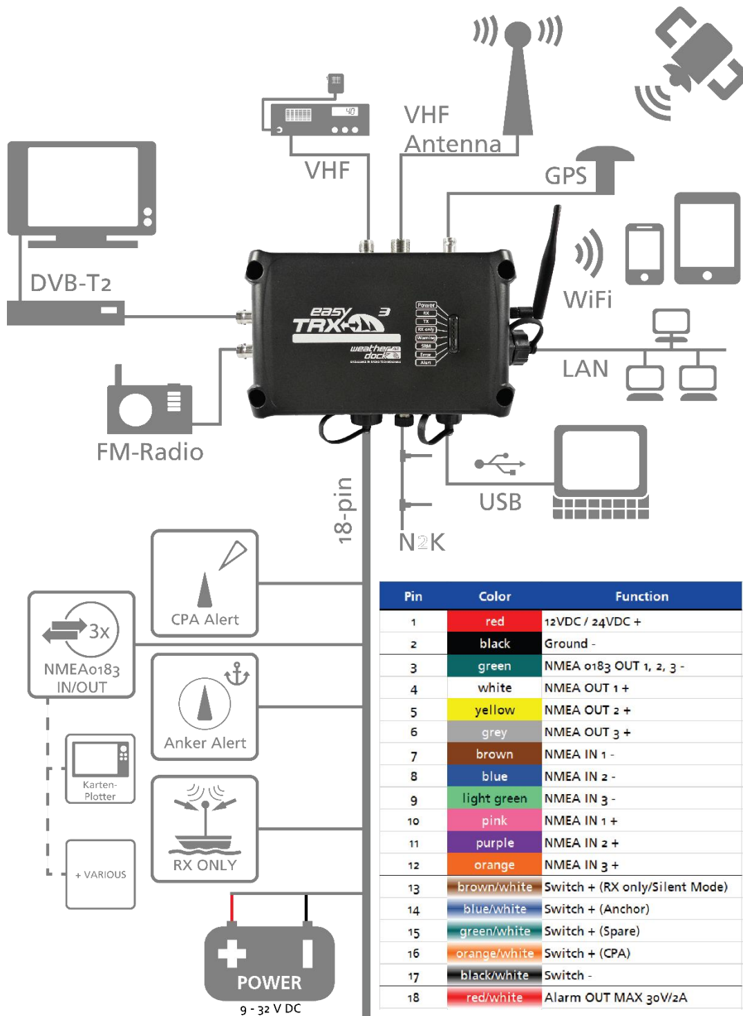
Figure: 3 Connection possibilities and cable colours
